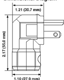
Dimensional Diagram
