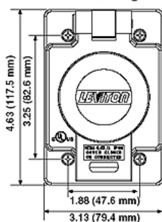
Dimensional Diagram
